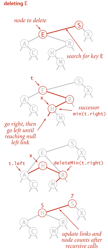
Deletion in a BST
