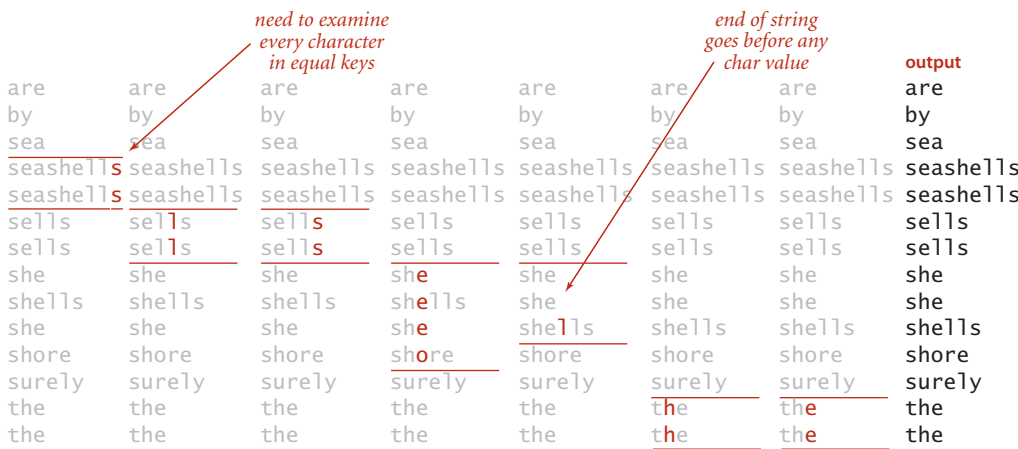
Trace of recursive calls for MSD string sort (no cutoff for small subarrays, subarrays of size 0 and 1 omitted)
