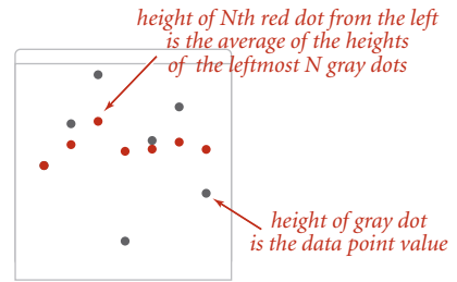
Visual accumulator plot
