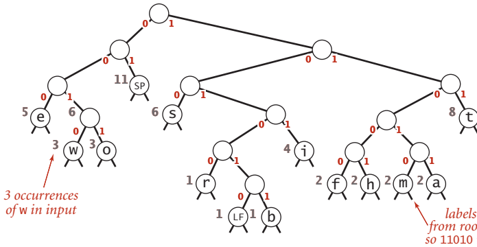
trie representation
