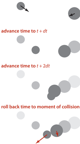
Time-driven simulation
