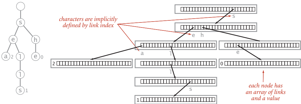
Trie representation ( R = 26 )
