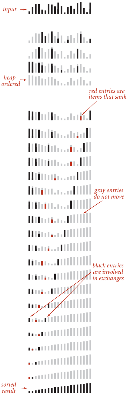
Visual trace of heapsort
