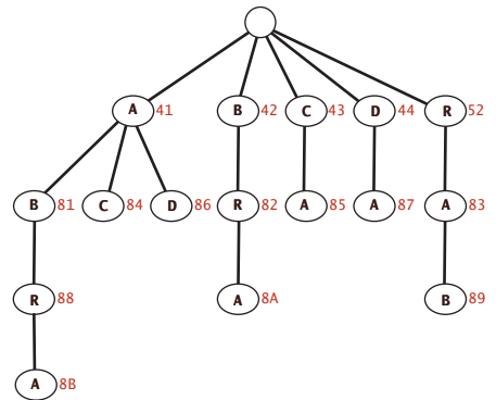
Trie representation of LZW code table
