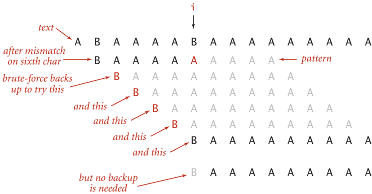
Text pointer backup in substrings searching
