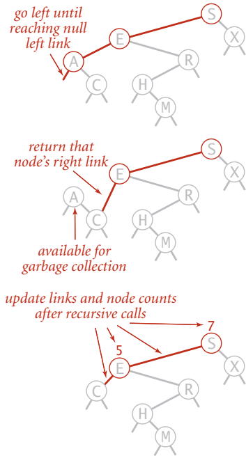
Deleting the minimum in a BST
