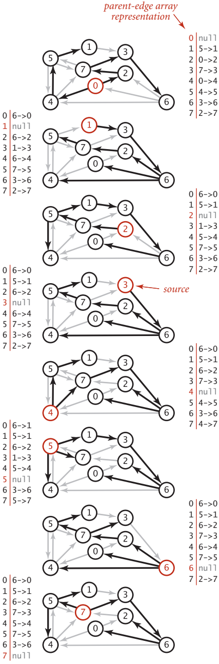
Shortest-paths trees
