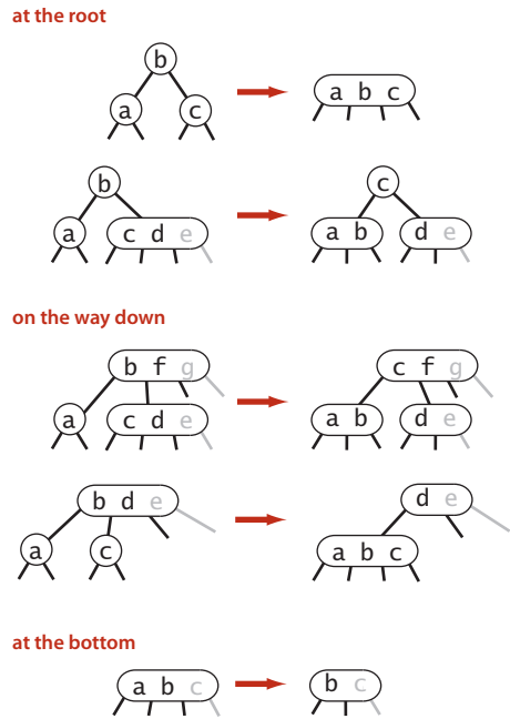
Transformations for delete the minimum
