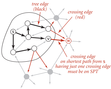
Dijkstra’s shortest-paths algorithm
