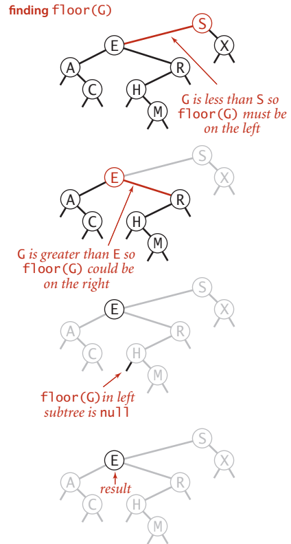
Computing the floor function
