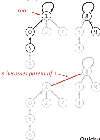
Quick-union overview
