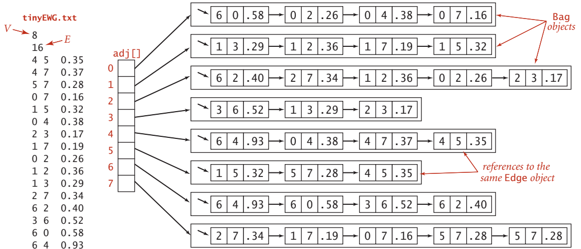
Edge-weighted graph representation
