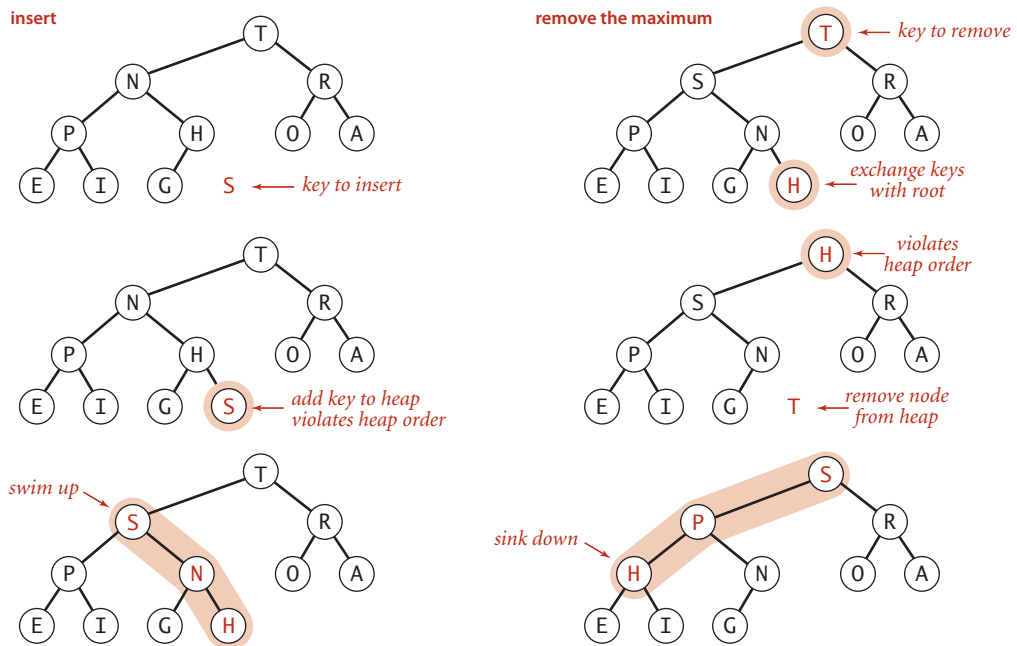
Heap operations
