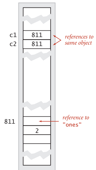
Aliasing
