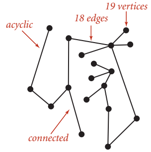
A tree
