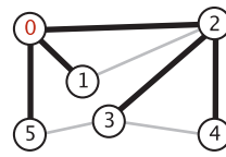
Outcome of breadth-first search to find all paths from 0
