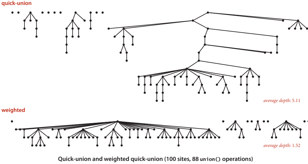
Quick-union and weighted quick-union (100 sites, 88 union() operations)
