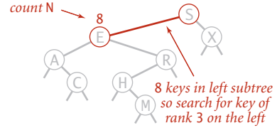
finding select(3) the key of rank 3
