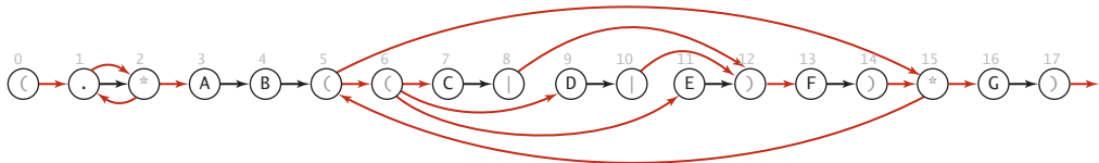
NFA corresponding to the pattern (.*AB((C|D|E)F)*G)
