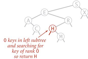
Selection in a BST
