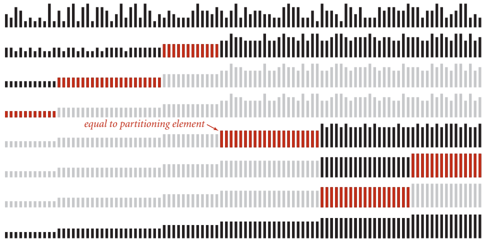
Visual trace of quicksort with 3-way partitioning
