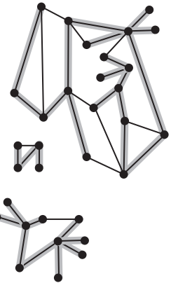
A spanning forest
