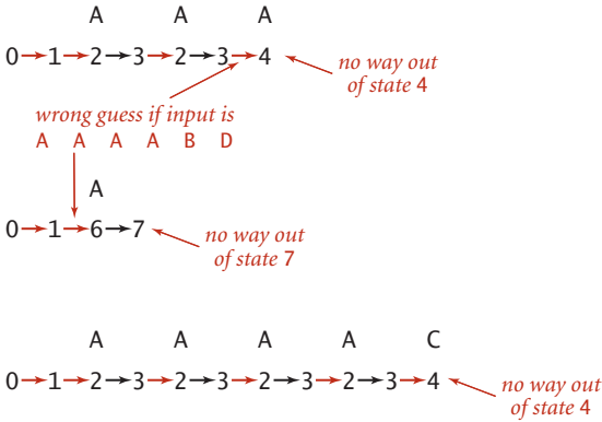
Stalling sequences for ( ( A * B | A C ) D ) NFA
