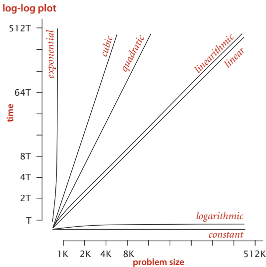
Typical orders of growth
