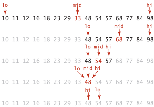
Binary search in an ordered array
